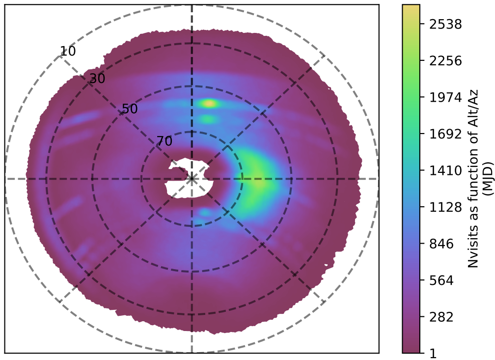
internal_u_expt27_nscale1.1v3.4_10yrs r band: Nvisits as function of Alt/Az
