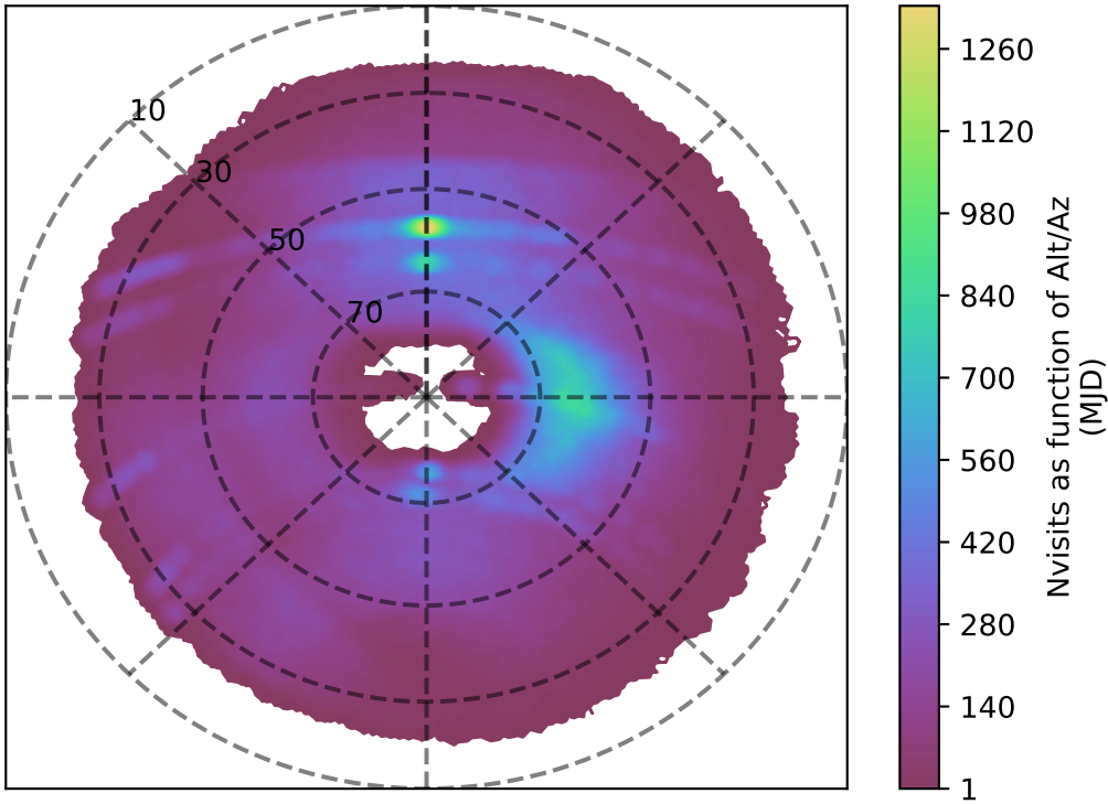
internal_u_expt27_nscale1.1v3.4_10yrs g band: Nvisits as function of Alt/Az
