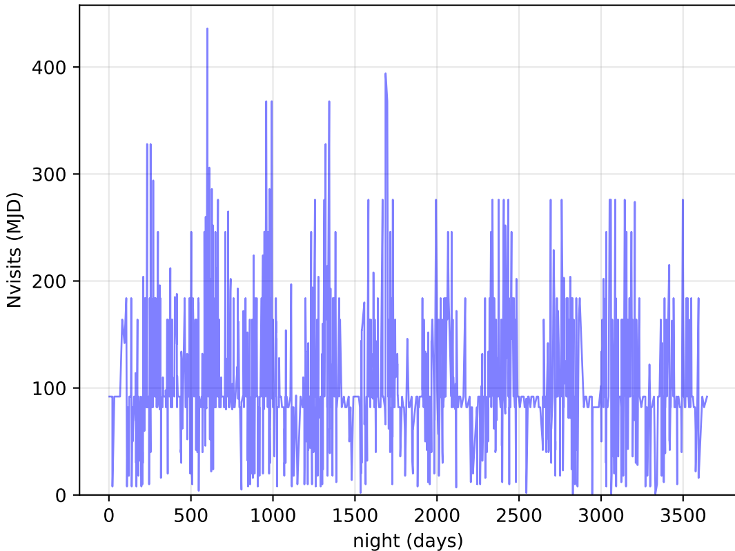
internal_u_expt27_nscale1.1v3.4_10yrs DDF: Nvisits
