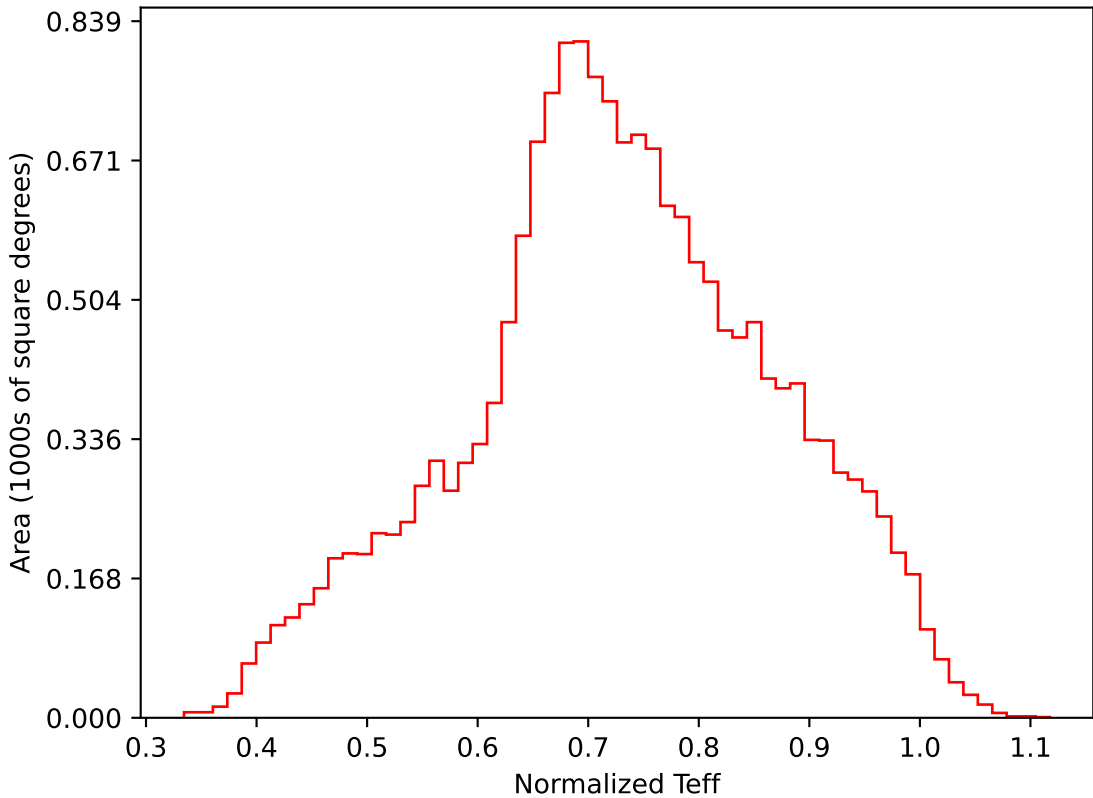
internal_u_expt27_nscale1.1v3.4_10yrs WFD i band: Normalized Teff
