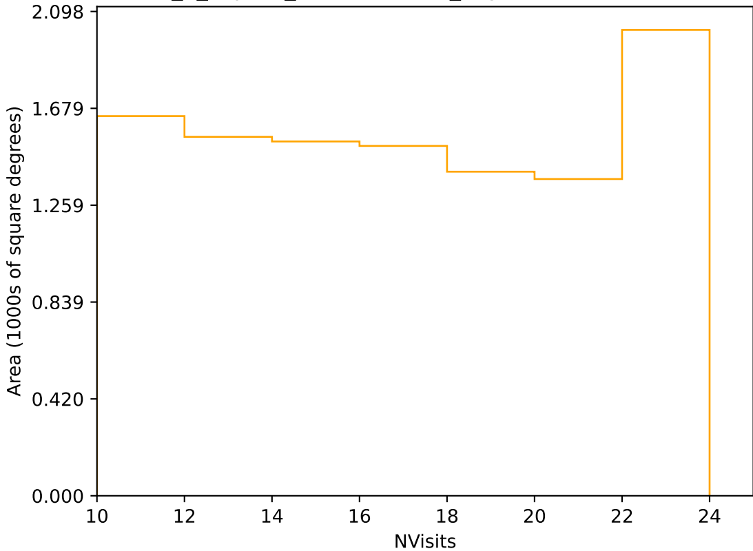
internal_u_expt27_nscale1.1v3.4_10yrs Yr 3-4 r band: NVisits
