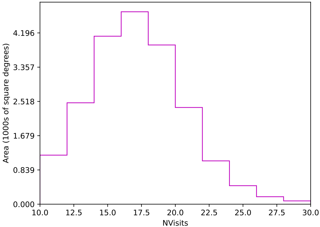
internal_u_expt27_nscale1.1v3.4_10yrs Yr 1 z band: NVisits
