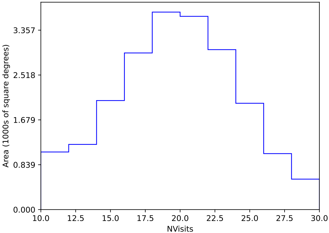
internal_u_expt27_nscale1.1v3.4_10yrs Yr 1 y band: NVisits
