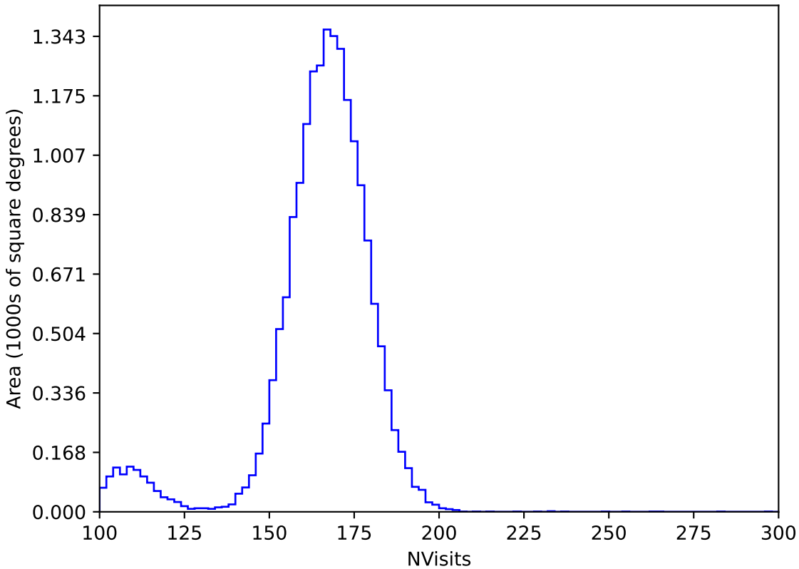
internal_u_expt27_nscale1.1v3.4_10yrs WFD y band: NVisits
