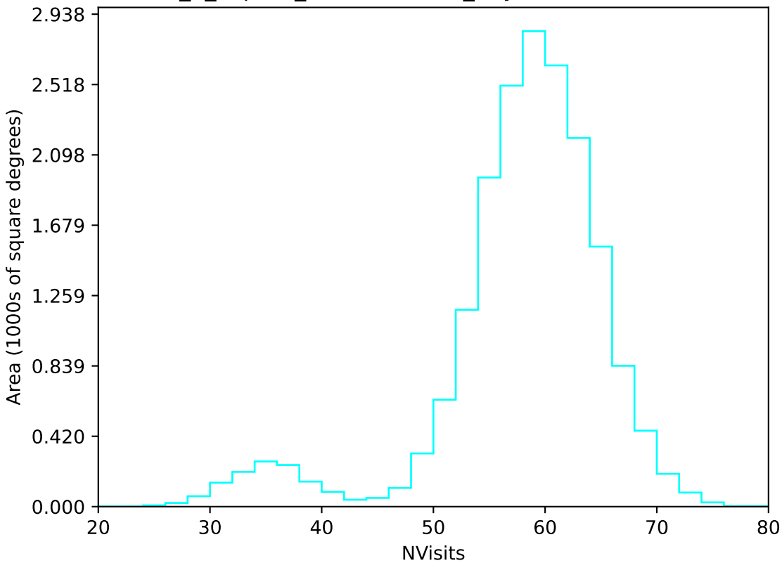
internal_u_expt27_nscale1.1v3.4_10yrs WFD u band: NVisits
