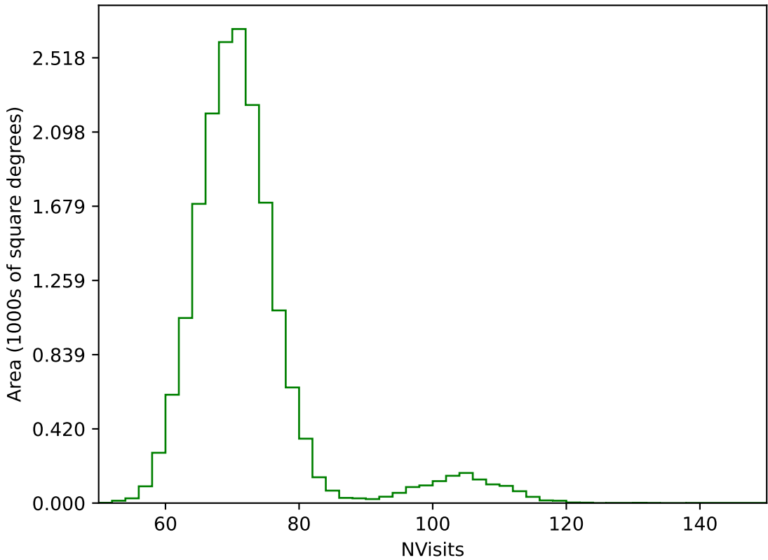
internal_u_expt27_nscale1.1v3.4_10yrs WFD g band: NVisits
