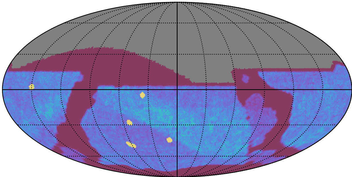
internal_u_expt27_nscale1.1v3.4_10yrs All sky z band: NVisits
