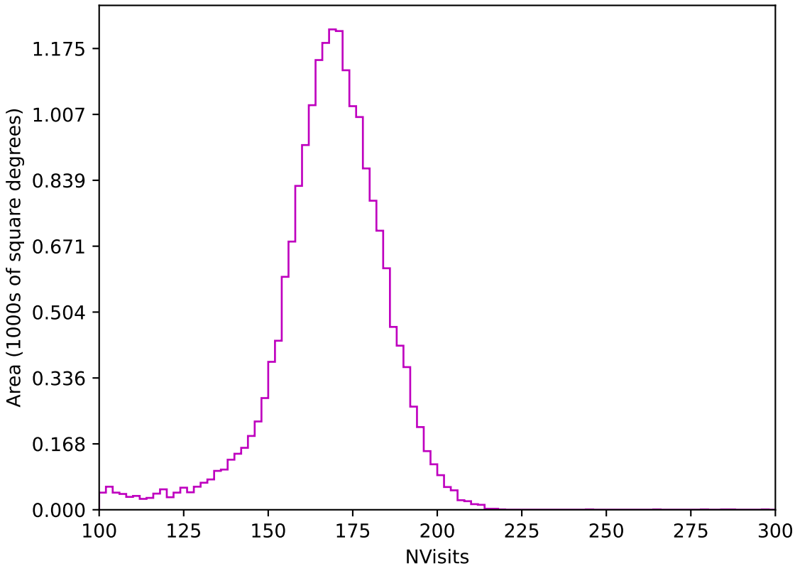
internal_u_expt27_nscale1.1v3.4_10yrs All sky z band: NVisits
