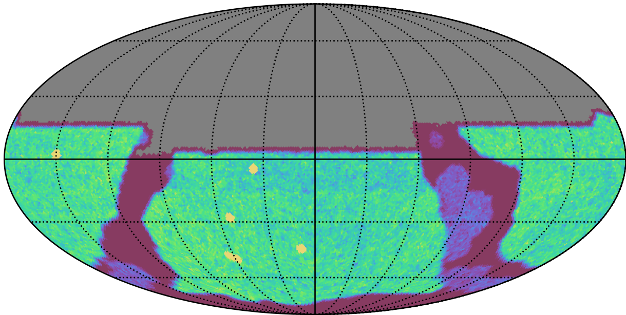
internal_u_expt27_nscale1.1v3.4_10yrs All sky u band: NVisits
