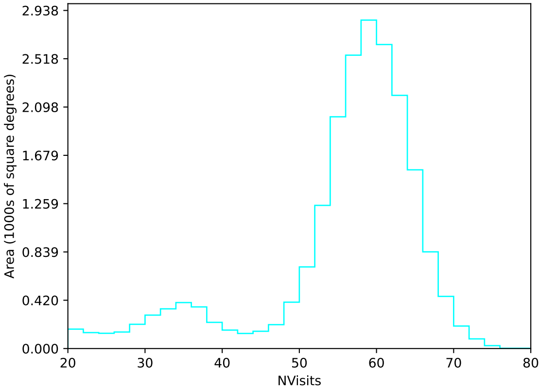
internal_u_expt27_nscale1.1v3.4_10yrs All sky u band: NVisits
