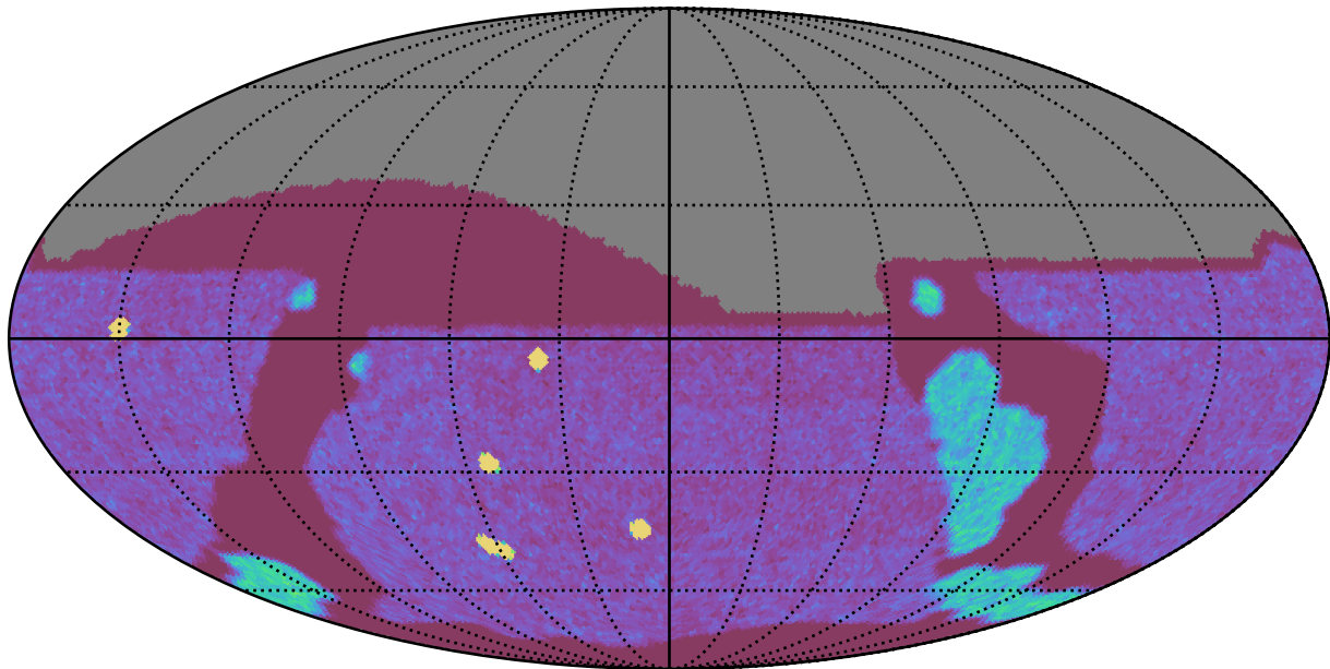
internal_u_expt27_nscale1.1v3.4_10yrs All sky g band: NVisits
