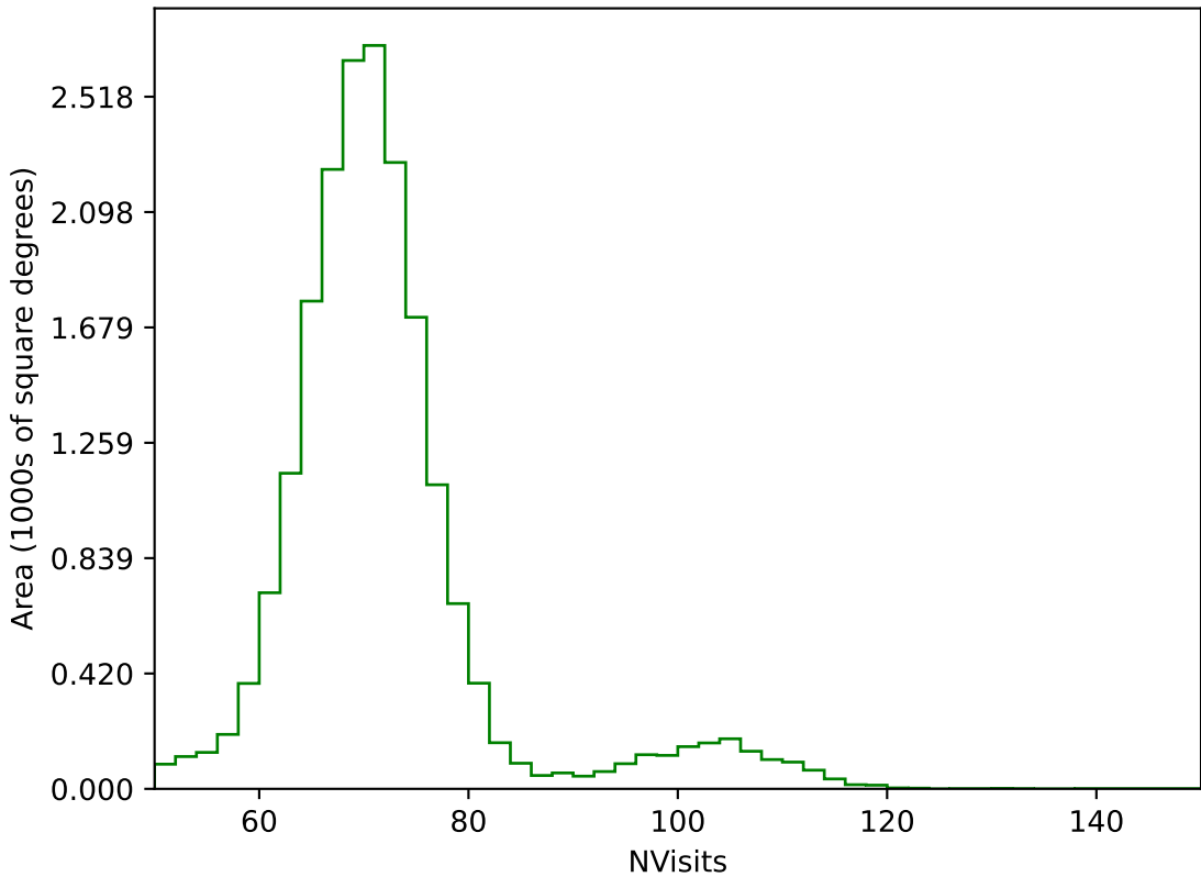
internal_u_expt27_nscale1.1v3.4_10yrs All sky g band: NVisits
