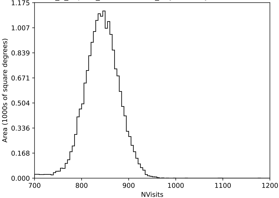
internal_u_expt27_nscale1.1v3.4_10yrs All sky all bands: NVisits
