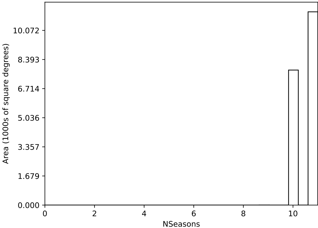
internal_u_expt27_nscale1.1v3.4_10yrs WFD all bands: NSeasons
