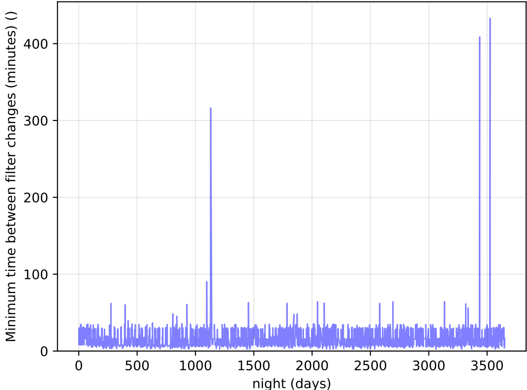
internal_u_expt27_nscale1.1v3.4_10yrs Per Night: Minimum time between filter changes (minutes)
