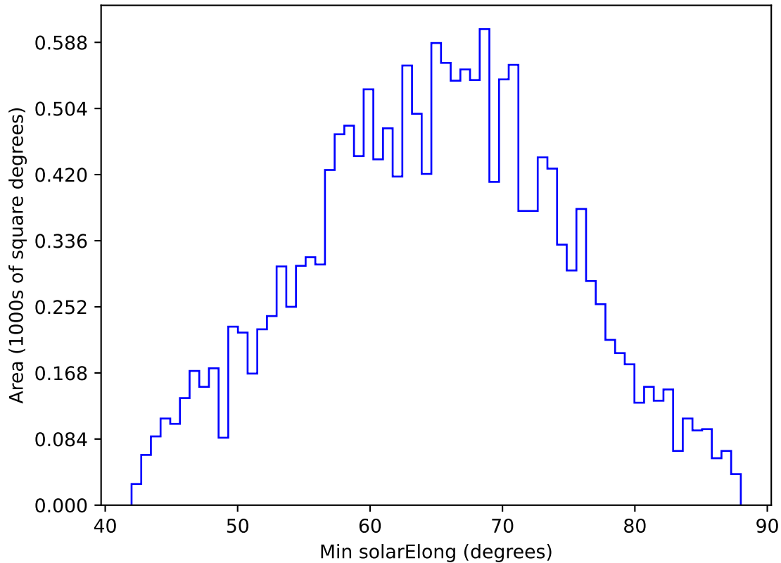
internal_u_expt27_nscale1.1v3.4_10yrs WFD y band: Min solarElong
