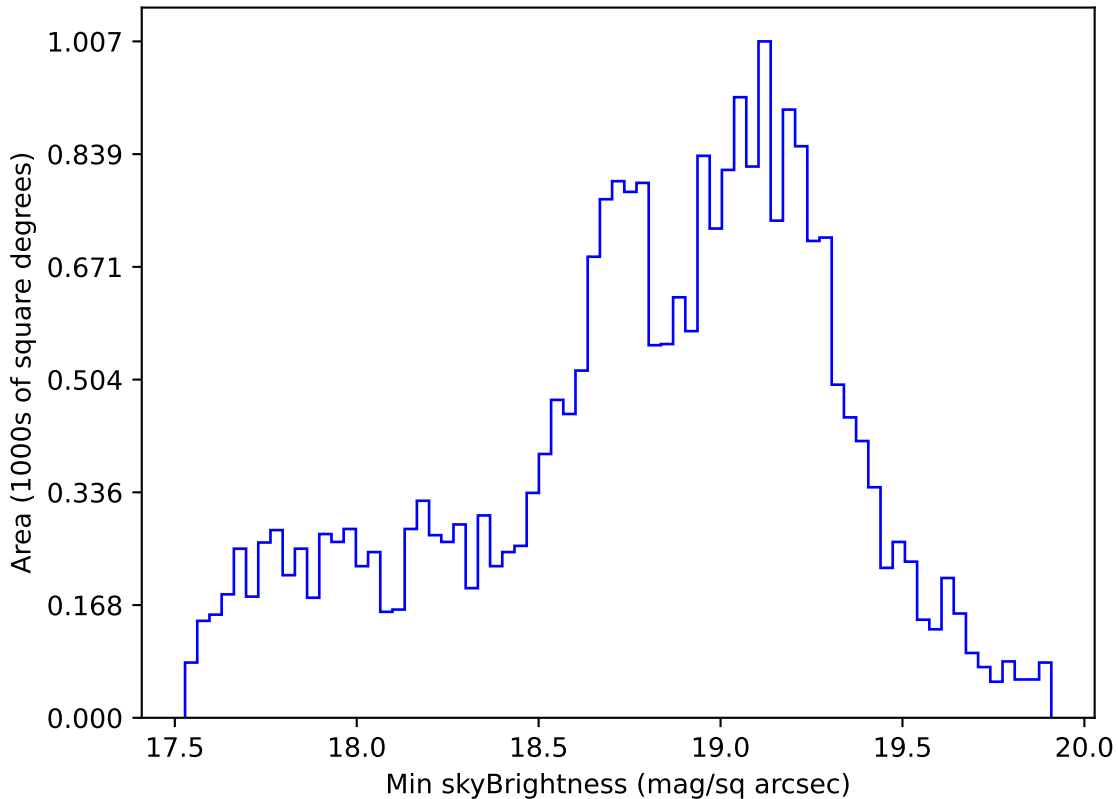
internal_u_expt27_nscale1.1v3.4_10yrs Yr 1 i band: Min skyBrightness
