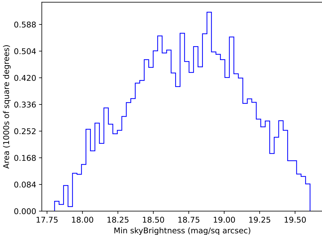
internal_u_expt27_nscale1.1v3.4_10yrs WFD r band: Min skyBrightness
