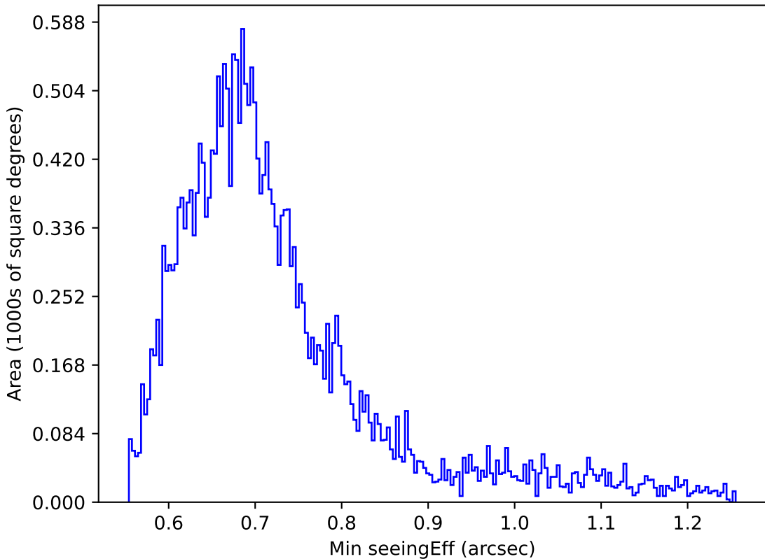
internal_u_expt27_nscale1.1v3.4_10yrs Yr 1 z band: Min seeingEff
