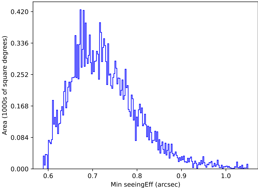
internal_u_expt27_nscale1.1v3.4_10yrs Yr 1 y band: Min seeingEff
