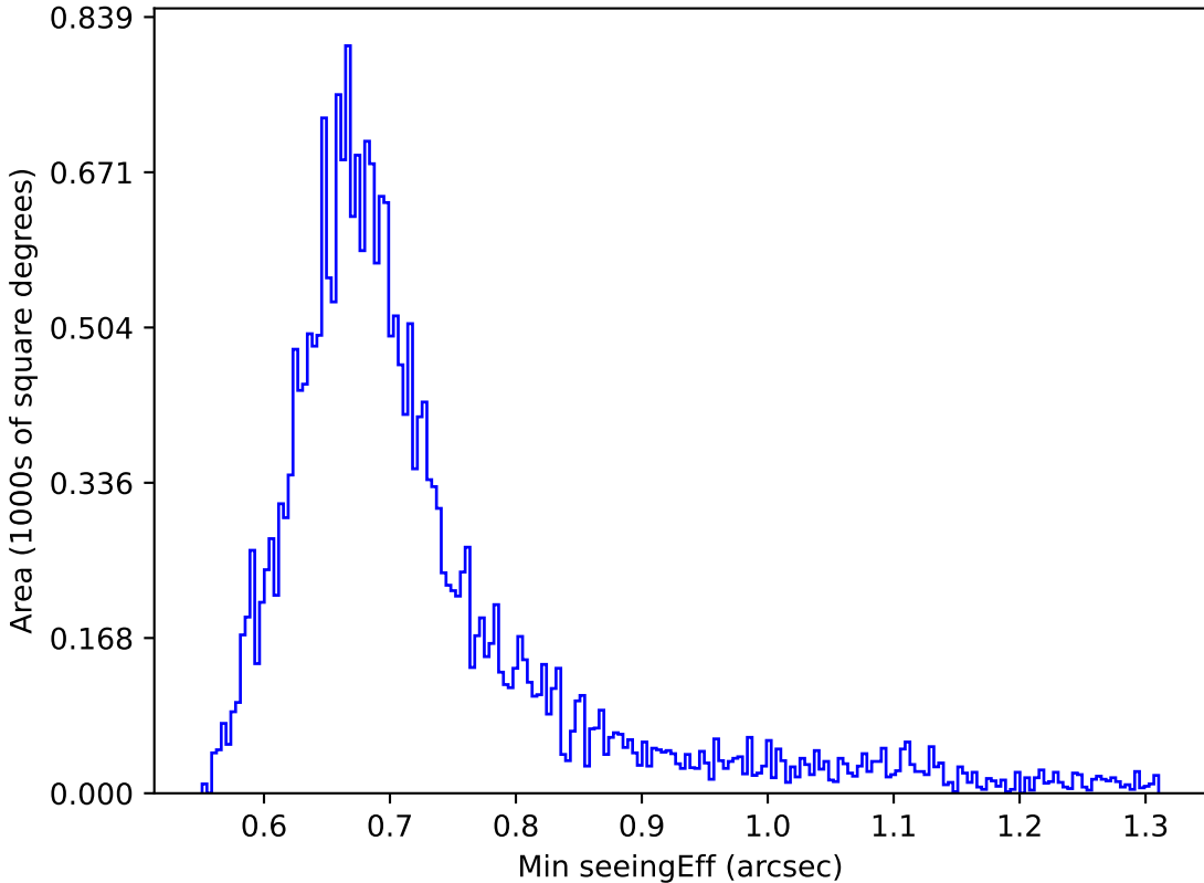
internal_u_expt27_nscale1.1v3.4_10yrs Yr 1 r band: Min seeingEff
