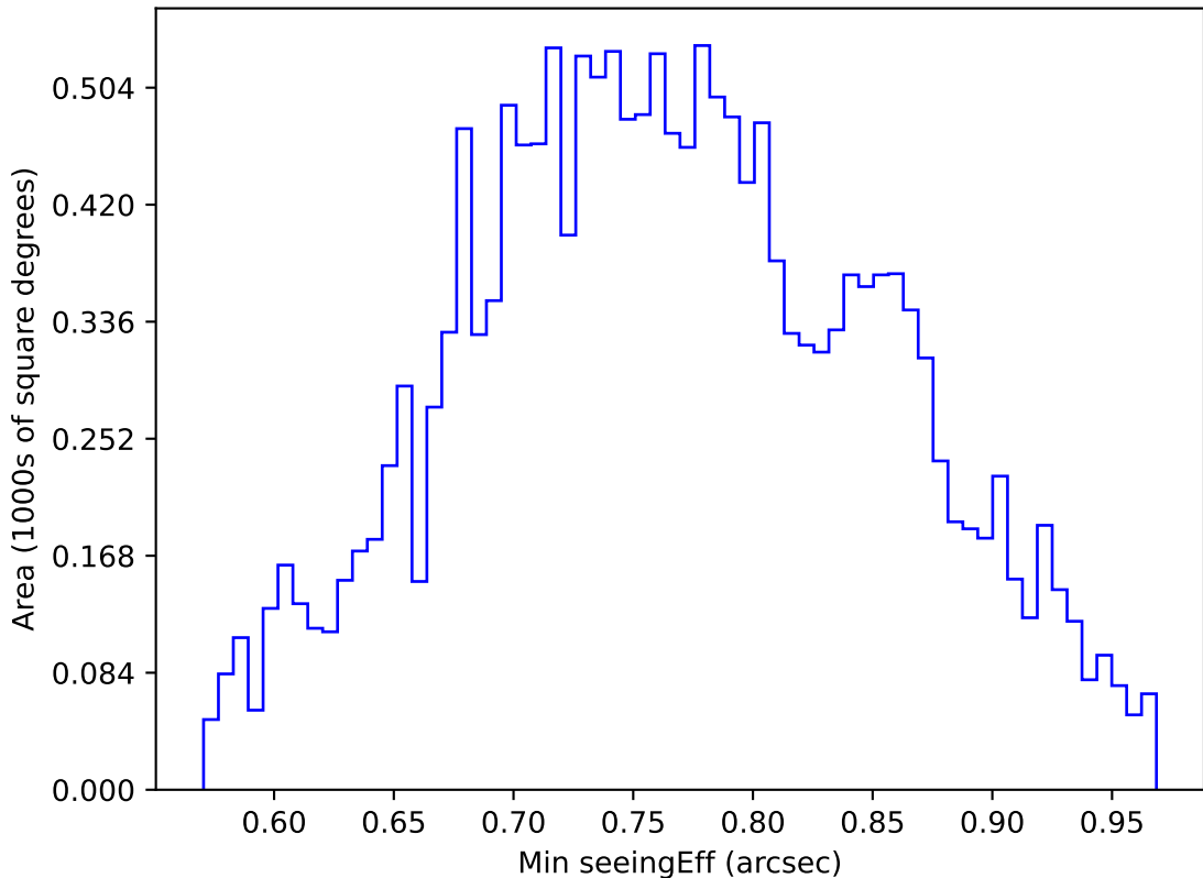
internal_u_expt27_nscale1.1v3.4_10yrs WFD u band: Min seeingEff
