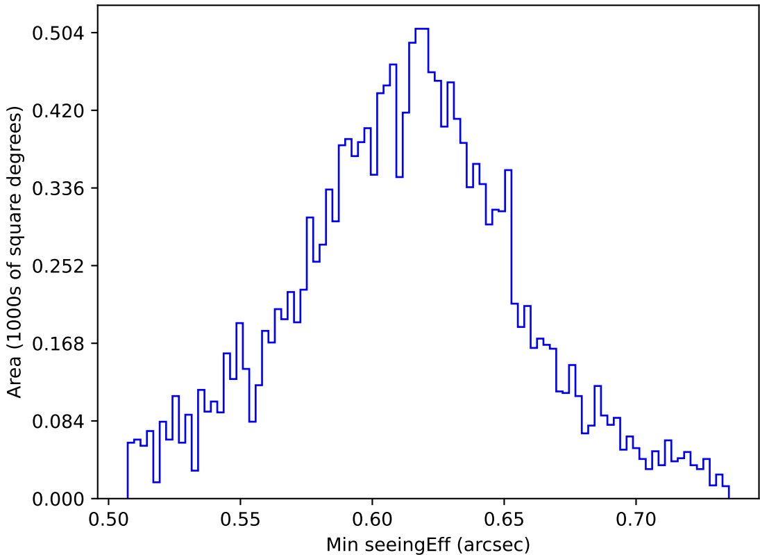
internal_u_expt27_nscale1.1v3.4_10yrs WFD r band: Min seeingEff
