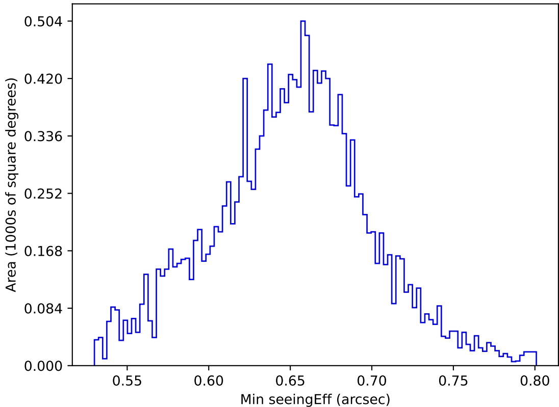
internal_u_expt27_nscale1.1v3.4_10yrs WFD g band: Min seeingEff
