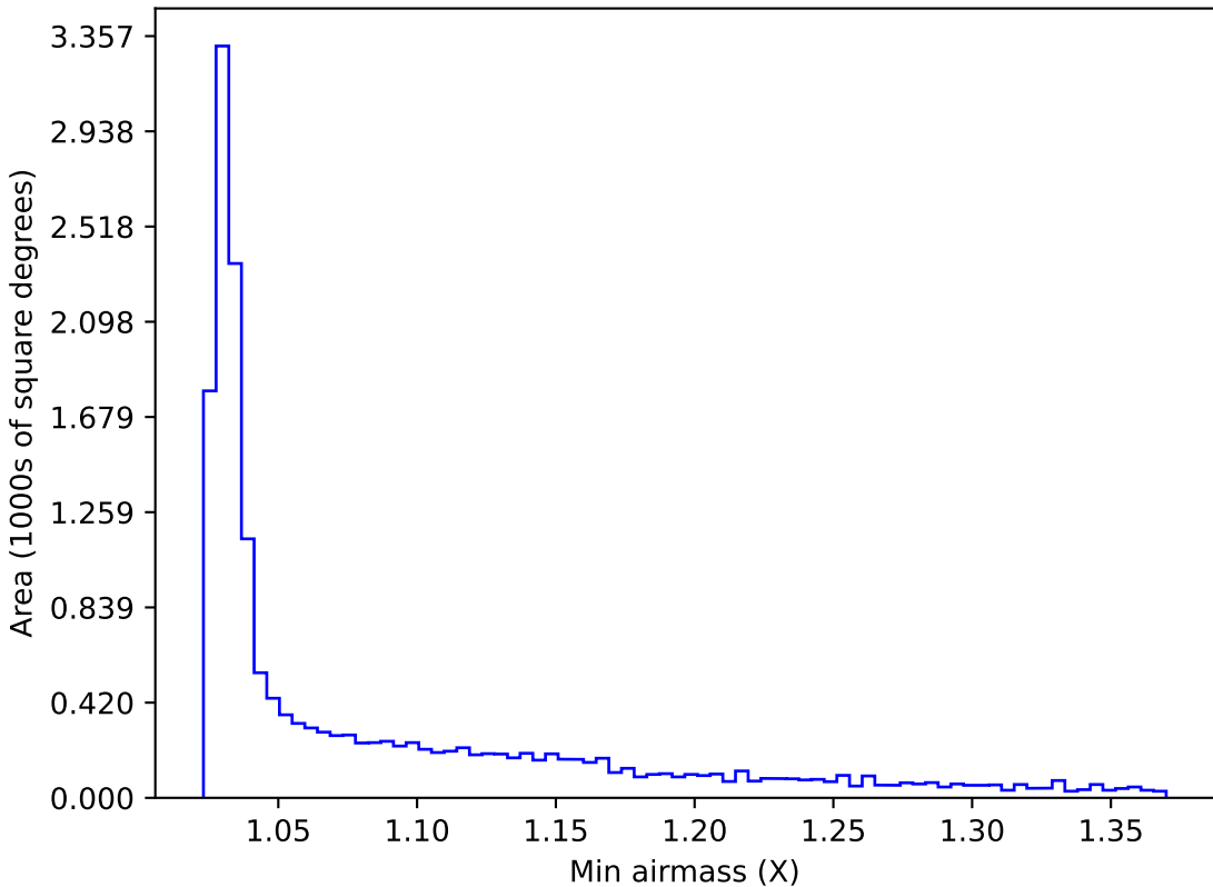
internal_u_expt27_nscale1.1v3.4_10yrs WFD y band: Min airmass
