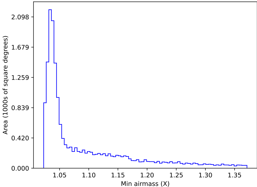
internal_u_expt27_nscale1.1v3.4_10yrs WFD g band: Min airmass
