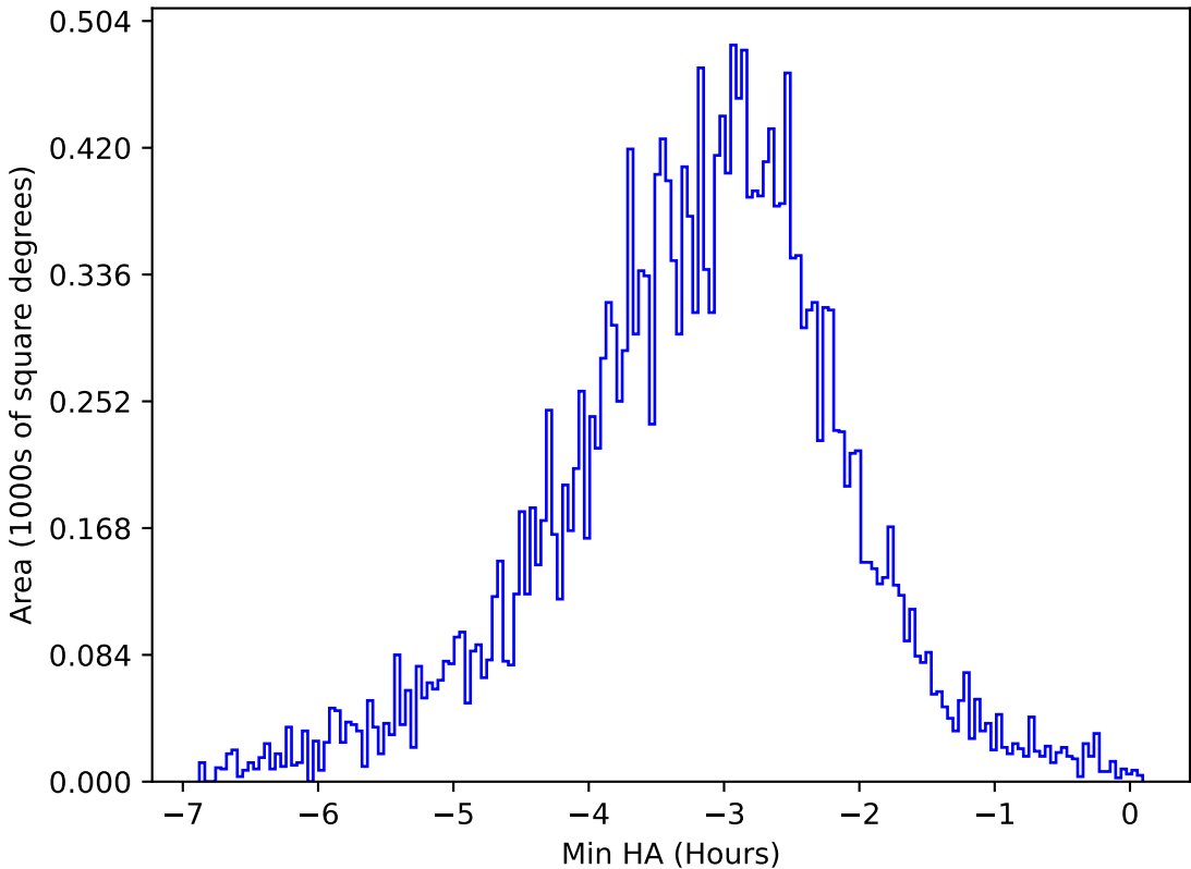
internal_u_expt27_nscale1.1v3.4_10yrs All sky u band: Min HA
