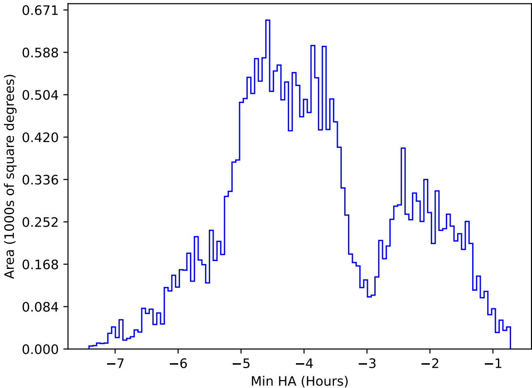
internal_u_expt27_nscale1.1v3.4_10yrs All sky g band: Min HA
