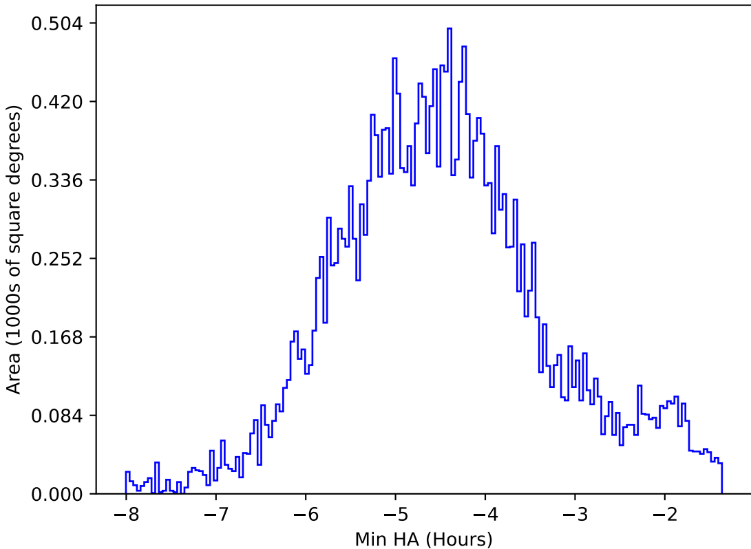
internal_u_expt27_nscale1.1v3.4_10yrs All sky all bands: Min HA
