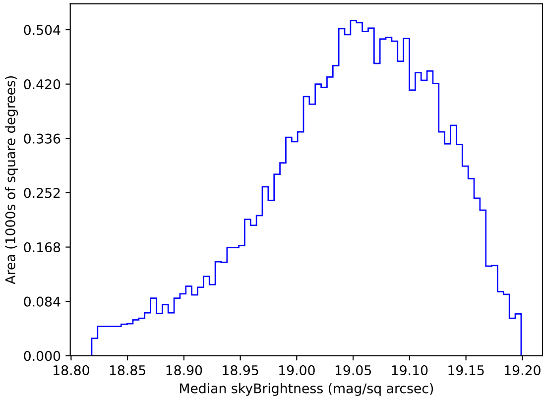
internal_u_expt27_nscale1.1v3.4_10yrs WFD z band: Median skyBrightness
