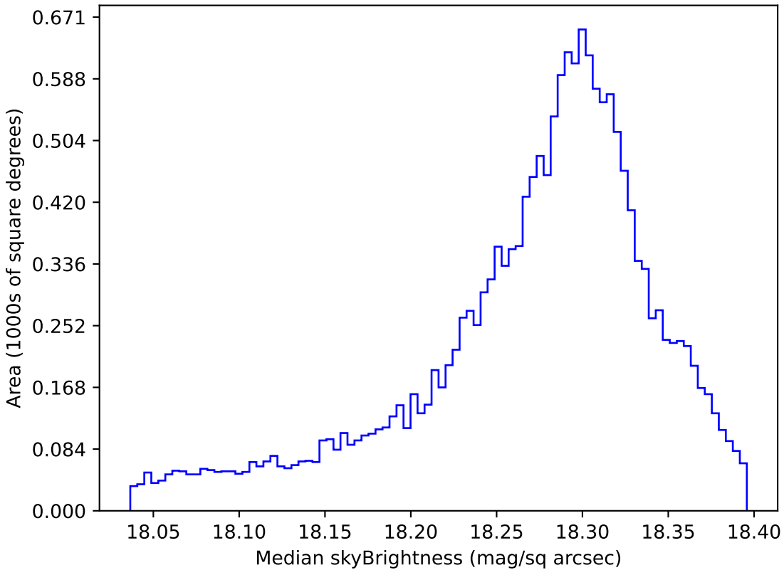
internal_u_expt27_nscale1.1v3.4_10yrs WFD y band: Median skyBrightness
