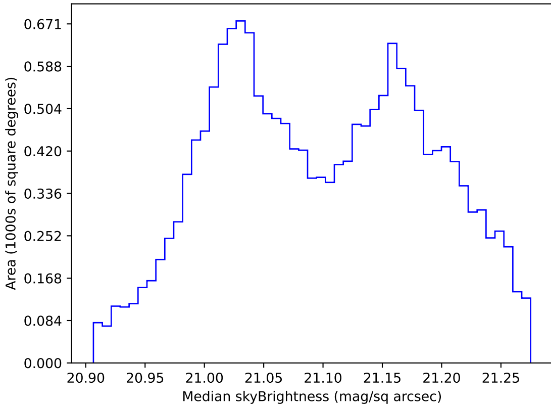
internal_u_expt27_nscale1.1v3.4_10yrs WFD r band: Median skyBrightness
