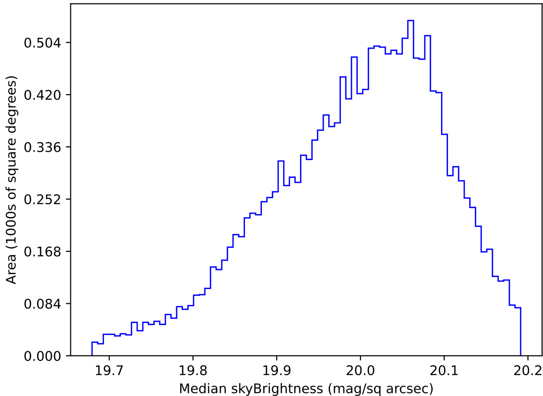
internal_u_expt27_nscale1.1v3.4_10yrs WFD i band: Median skyBrightness
