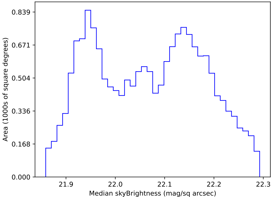
internal_u_expt27_nscale1.1v3.4_10yrs WFD g band: Median skyBrightness
