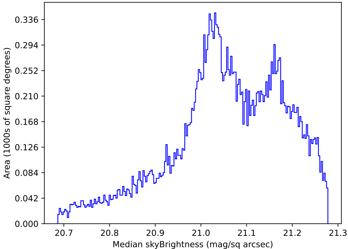
internal_u_expt27_nscale1.1v3.4_10yrs All sky r band: Median skyBrightness
