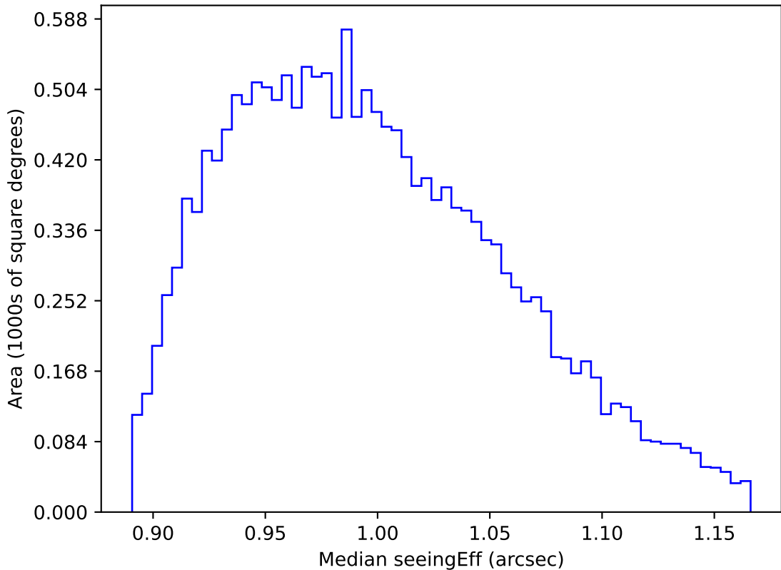
internal_u_expt27_nscale1.1v3.4_10yrs WFD y band: Median seeingEff
