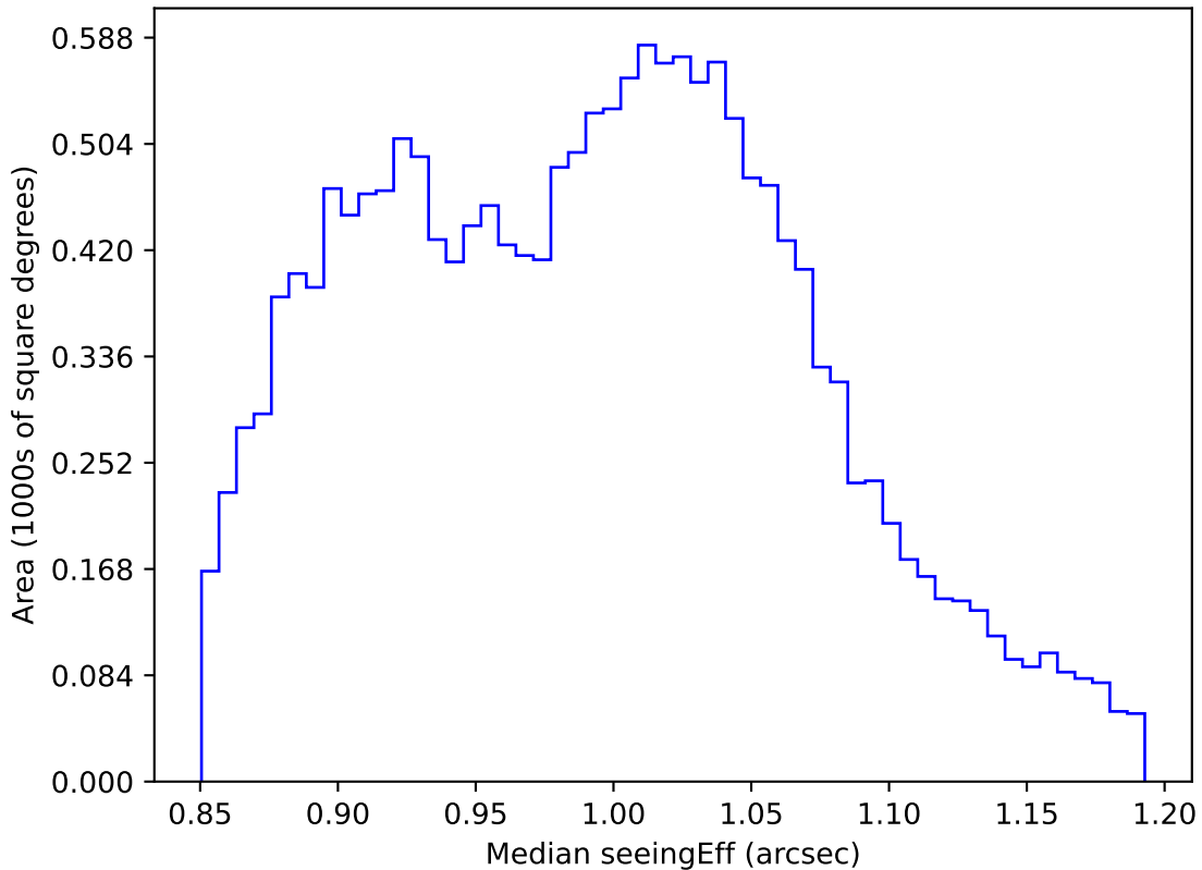
internal_u_expt27_nscale1.1v3.4_10yrs WFD i band: Median seeingEff
