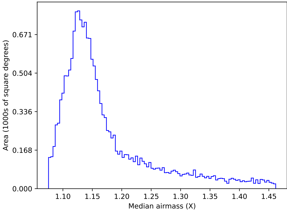
internal_u_expt27_nscale1.1v3.4_10yrs WFD r band: Median airmass
