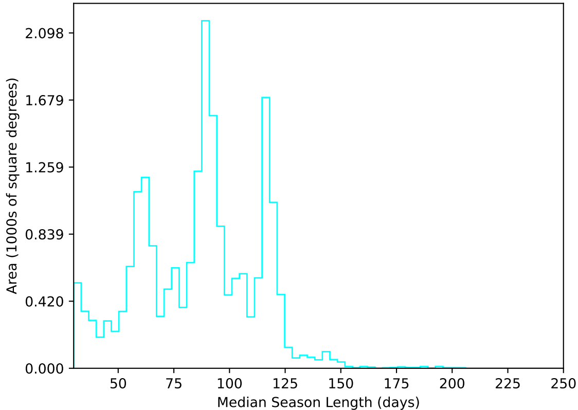
internal_u_expt27_nscale1.1v3.4_10yrs All sky u band: Median Season Length
