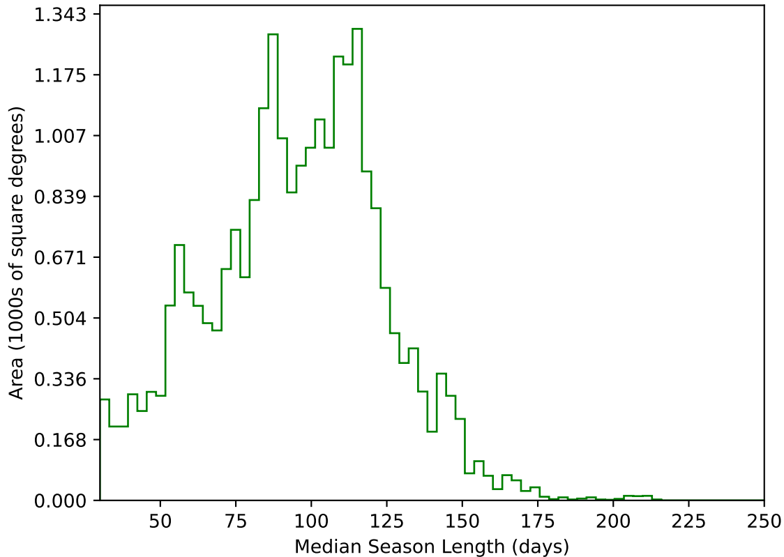
internal_u_expt27_nscale1.1v3.4_10yrs All sky g band: Median Season Length
