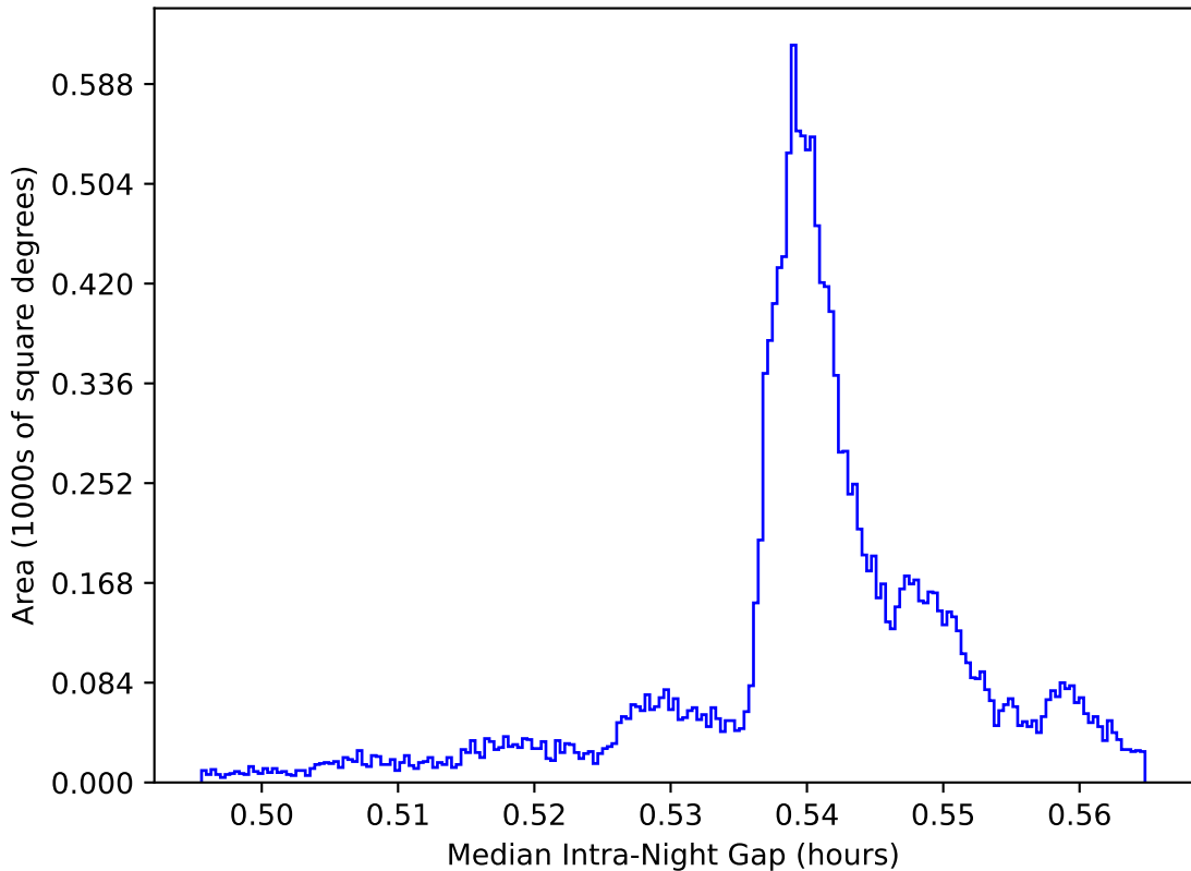
internal_u_expt27_nscale1.1v3.4_10yrs WFD: Median Intra-Night Gap
