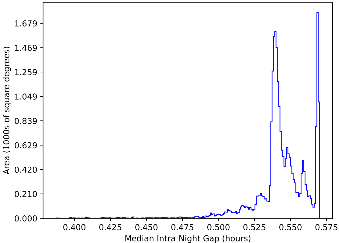
internal_u_expt27_nscale1.1v3.4_10yrs All sky: Median Intra-Night Gap
