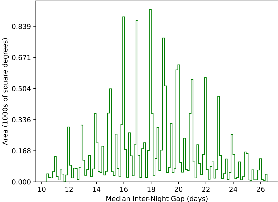
internal_u_expt27_nscale1.1v3.4_10yrs WFD g band: Median Inter-Night Gap
