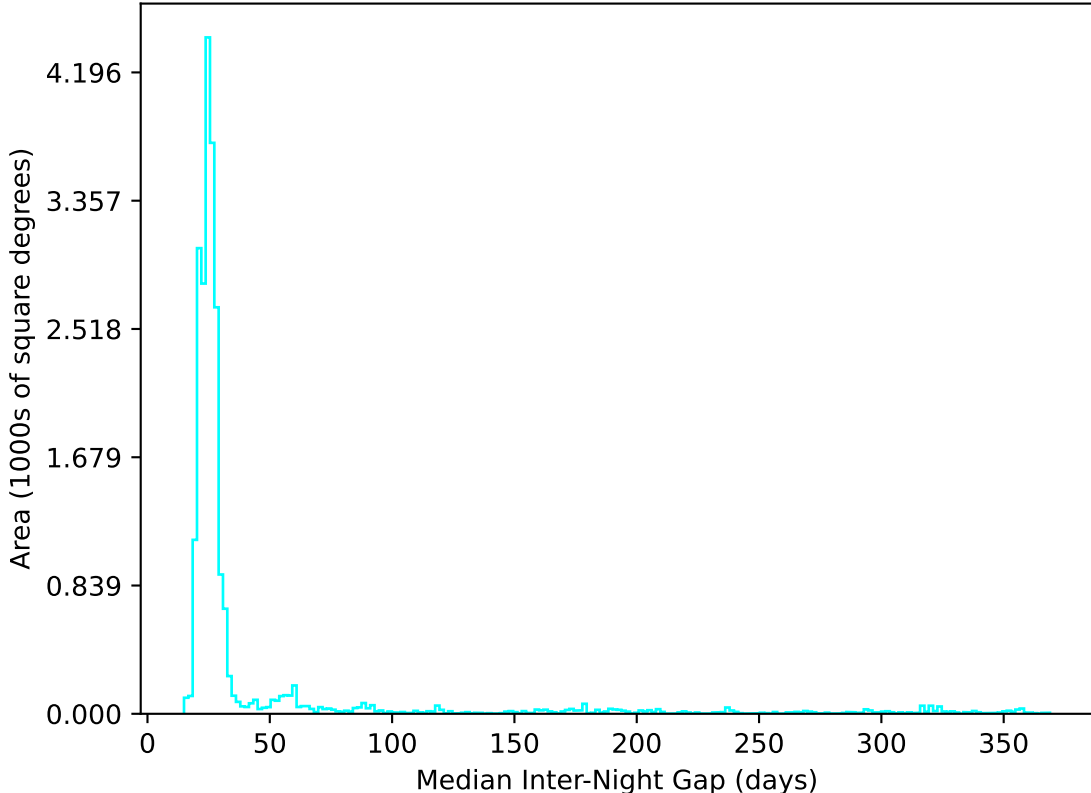
internal_u_expt27_nscale1.1v3.4_10yrs All sky u band: Median Inter-Night Gap
