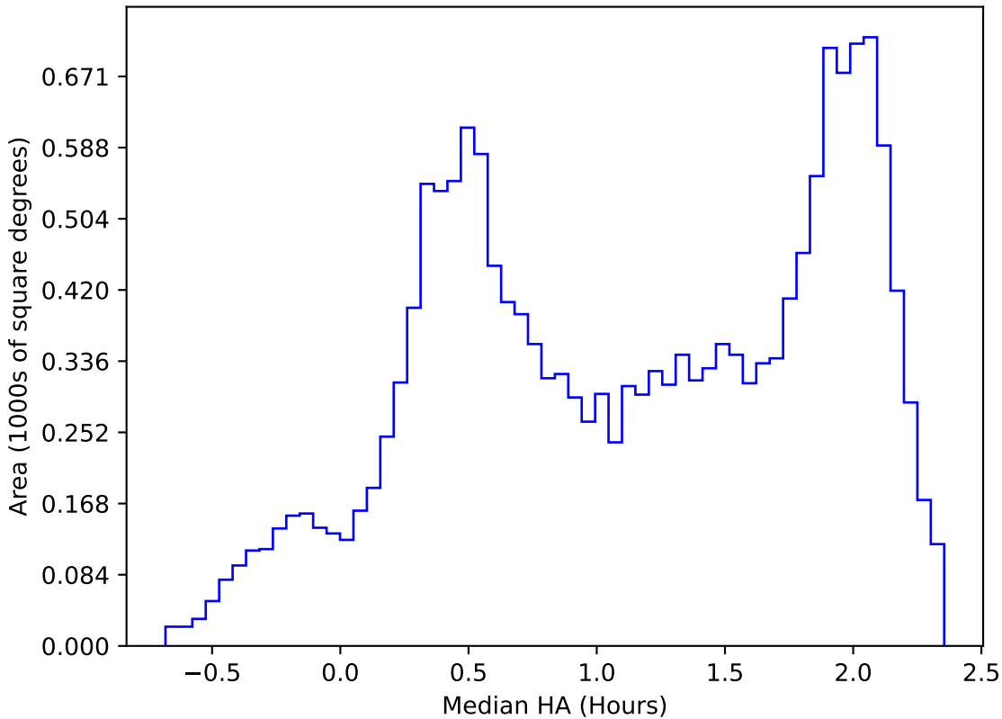
internal_u_expt27_nscale1.1v3.4_10yrs WFD z band: Median HA
