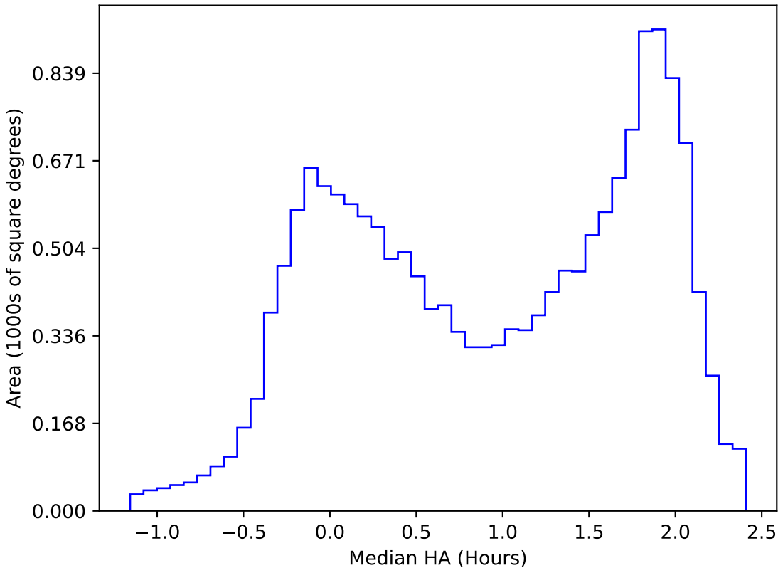
internal_u_expt27_nscale1.1v3.4_10yrs WFD u band: Median HA
